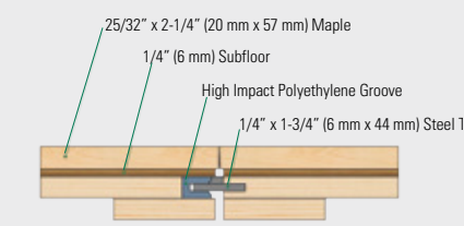
TONGUE & GROOVE DETAIL
