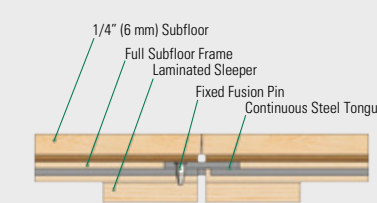
QUICK PIN DETAIL
