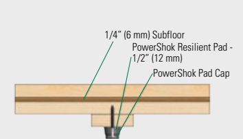
POWERSHOK PAD (OPTIONAL ACCESSORY)
